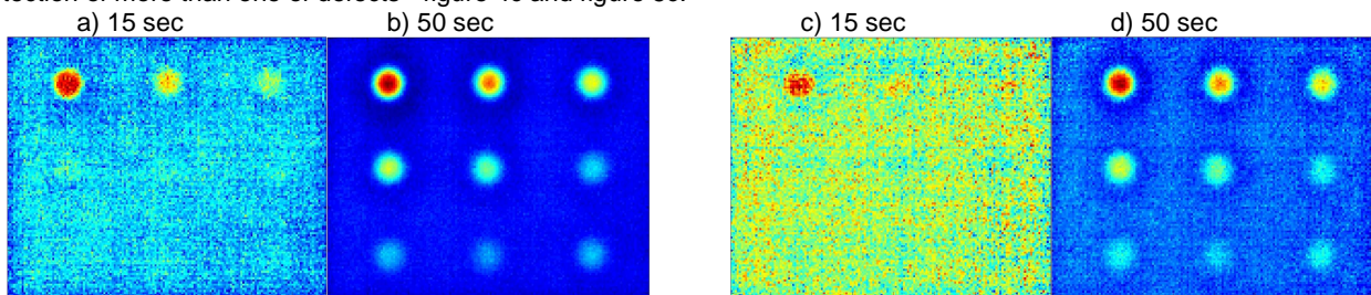
Fig. 5. Filtered contrast FC for: a-b) symmetric excitation (left and right lamp), c-d) for asymmetric excitation (only right lamp)
