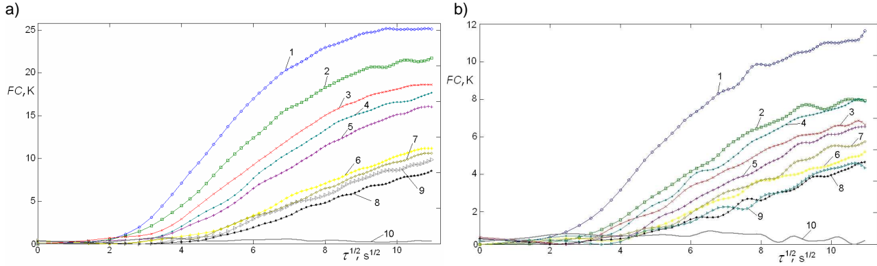
Fig. 6. Filtered contrast FC as a function of square root of time for the midpoints of areas 1-10: a) symmetric excitation (left and right lamp), b) for asymmetric excitation (only right lamp)
