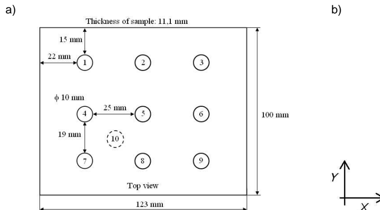
Fig. 2. a) Geometry of tested sample, where: 1-9 – defects, 10 – sound area, b) XY coordinates
