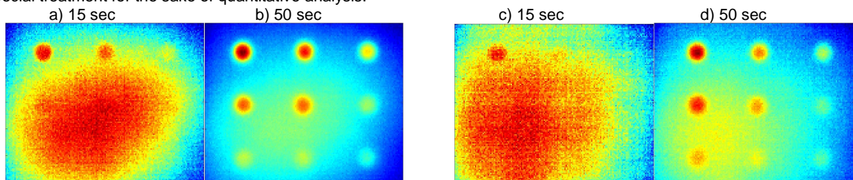
Fig. 4. Raw thermograms for: a-b) symmetric excitation (left and right lamp), c-d) for asymmetric excitation (only right lamp)
